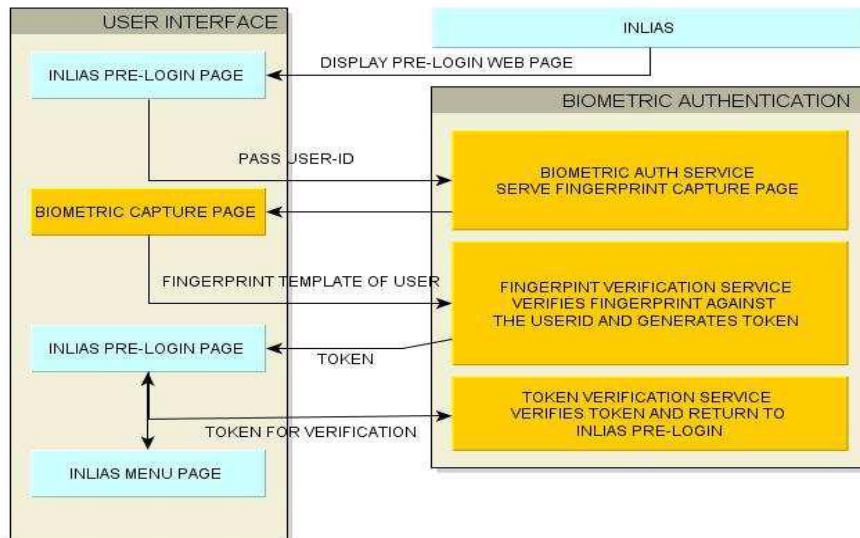
Fig: Flow chart for INLAIS -TOKEN verification service
