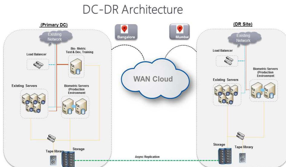
Fig: DC to DR Replication
