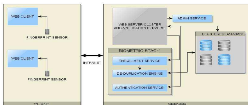
Fig: Client Server Architecture for BAS
